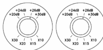
Figure 3 – H-3000 Chassis Top View - MC Transformer Controls
