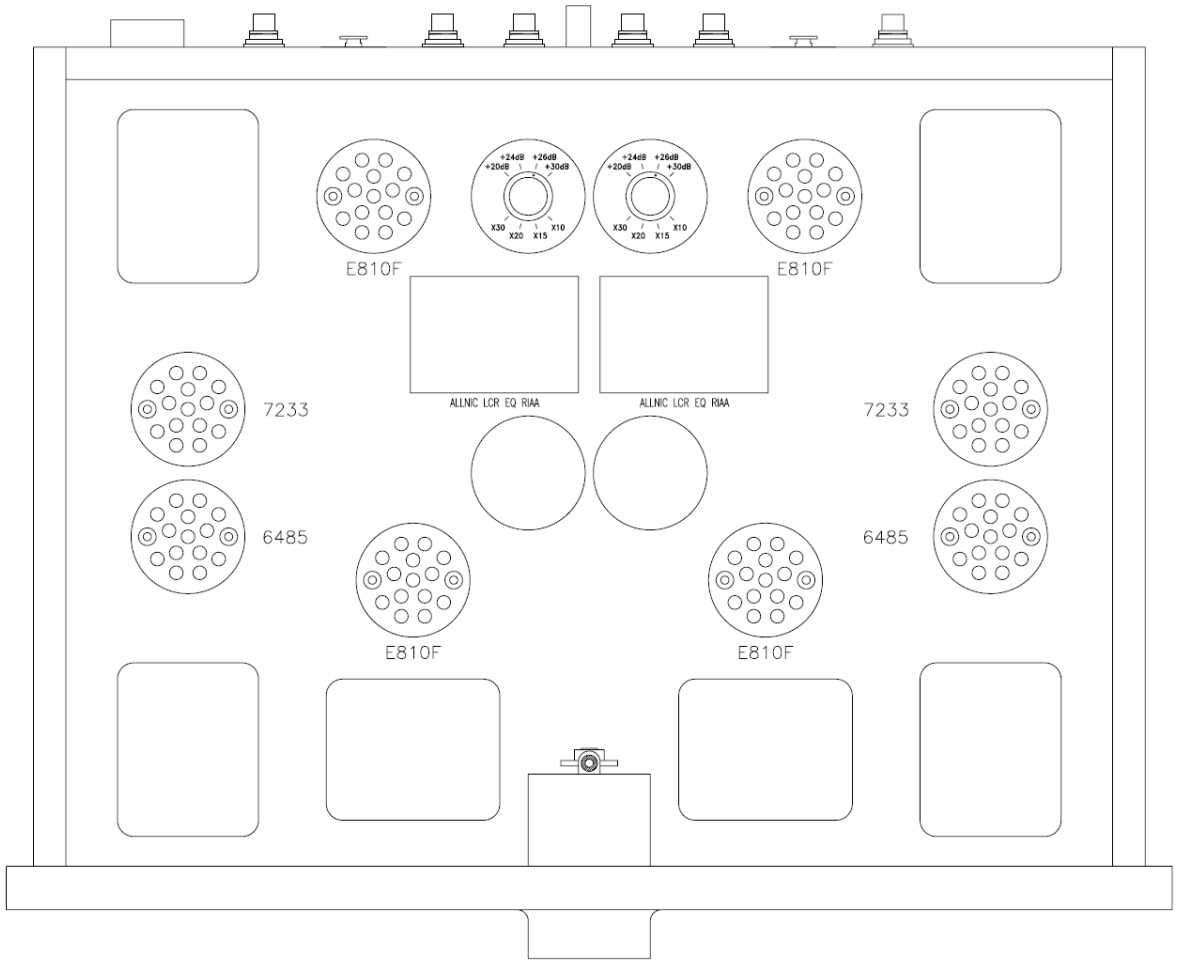
Figure 6 – H-3000 Internal View
