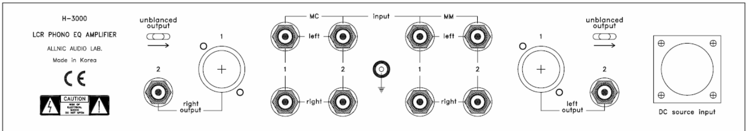
Figure 1 – H-3000 Rear Panel View
